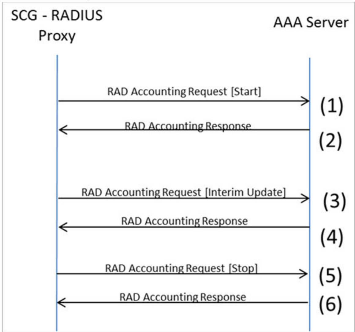
FIGURE 7 RADIUS Accounting call flow
